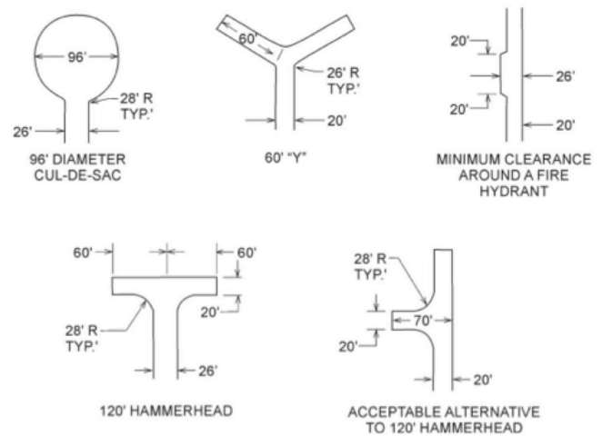
Figure 6. Recommended turn-arounds for fire engines (by Oregon State www.iccsafe.org/ ).
